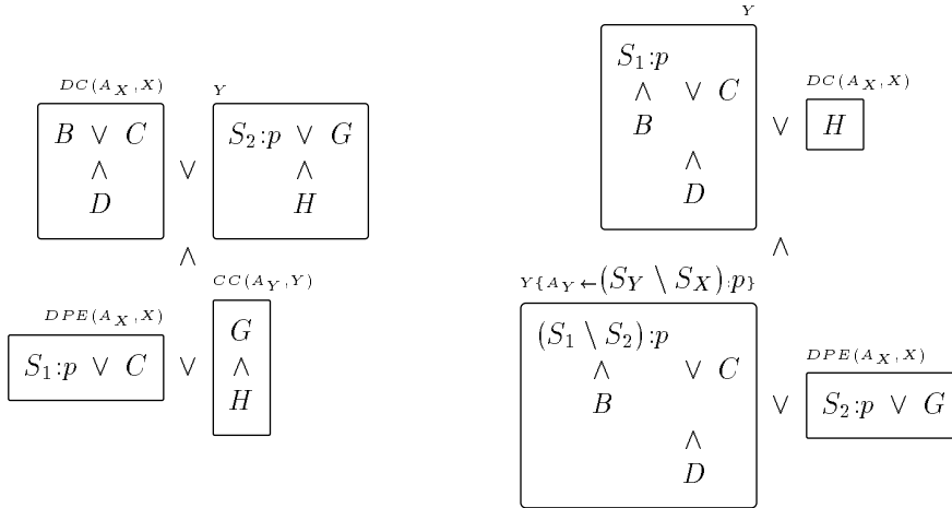
Fig. 3. The two possible results of applying the anti-link operator to F if S_2 \subseteq S_1 , S_1 \not\subseteq S_2 .
